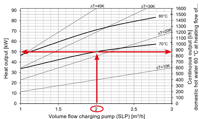
Domestic hot water continuous output at 60 °C
