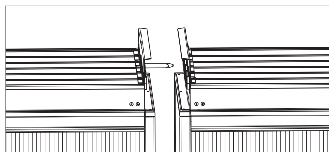
Fig. D5: Connecting bolts for damper connection for partitioned exchangers
